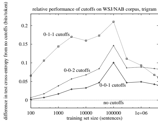
Figure 35: Performance relative to model with no count cutoffs of models with cutoffs on WSJ/NAB corpus, jelinek-mercer-smoothing , bigram and trigram models
