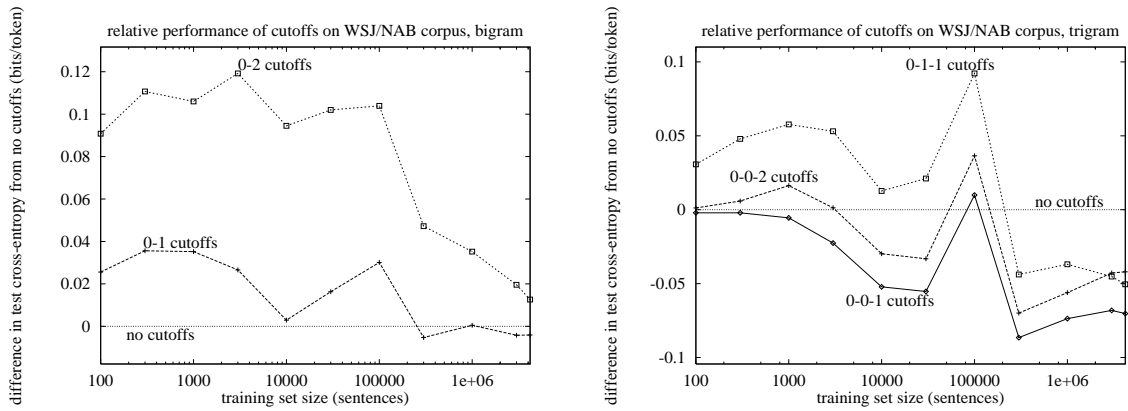
Figure 35: Performance relative to model with no count cutoffs of models with cutoffs on WSJ/NAB corpus, jelinek-mercer-smoothing , bigram and trigram models
